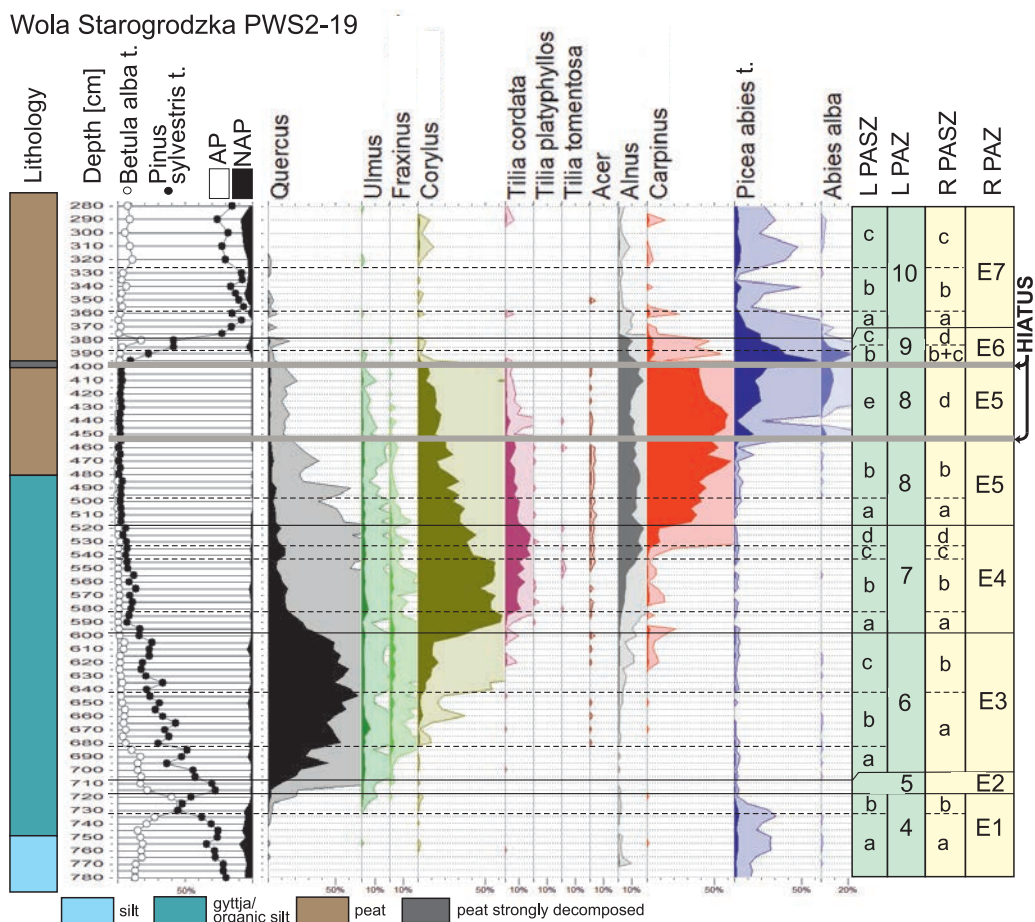
Text-fig. 4. Wola Starogrodzka PWS2-19 profile. Simplified pollen percentage diagram. Regional pollen assemblage zones (R PAZ) according to Mamakowa (1989), and subzones (R PASZ) according to Kupryjanowicz and Granoszewski (2018).
